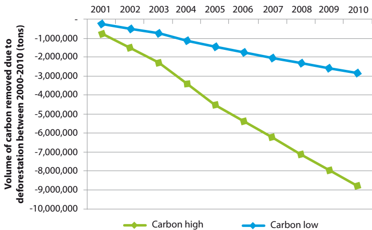
Figure 5.7: Reduction in above-ground carbon storage capacity in Kenya due to deforestation between 2000 and 2010.
