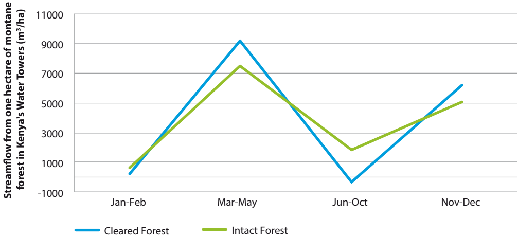
Figure 4.2: Changes in long-term seasonal flow distribution of one hectare of intact and cleared montane forest areas in Kenya's Water Towers
